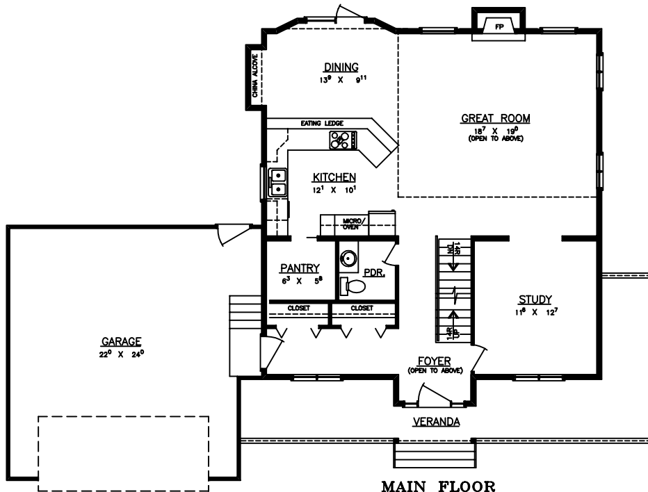
MAIN FLOOR AREA = 1095 S.F.
