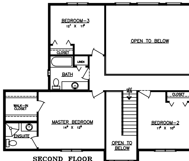
SECOND FLOOR AREA = 795 S.F.
